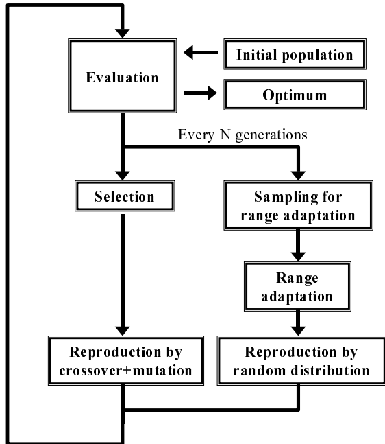
Figure 3. Flow chart of the present ARGAs.
