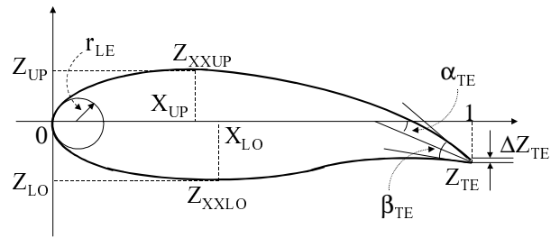
Figure 5. Design parameters for the Sobieczky shape functions.
