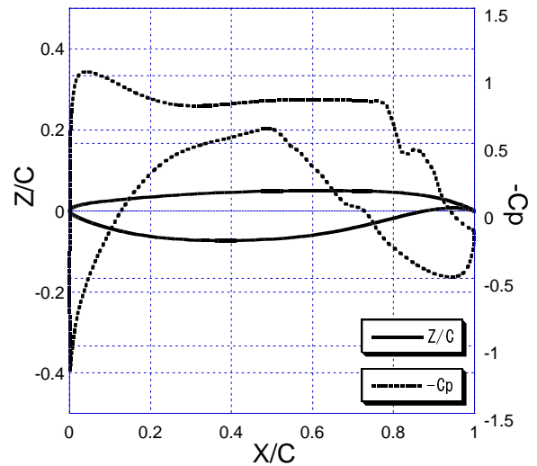
Figure 7. Designed airfoil shape and the corresponding pressure distribution.
